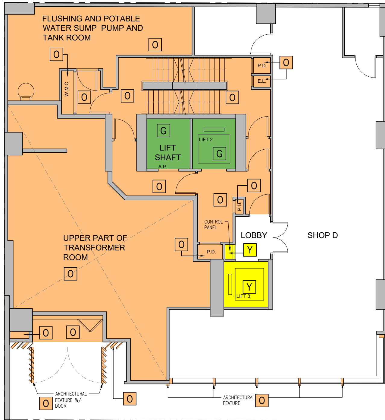
2/F FLOOR PLAN
