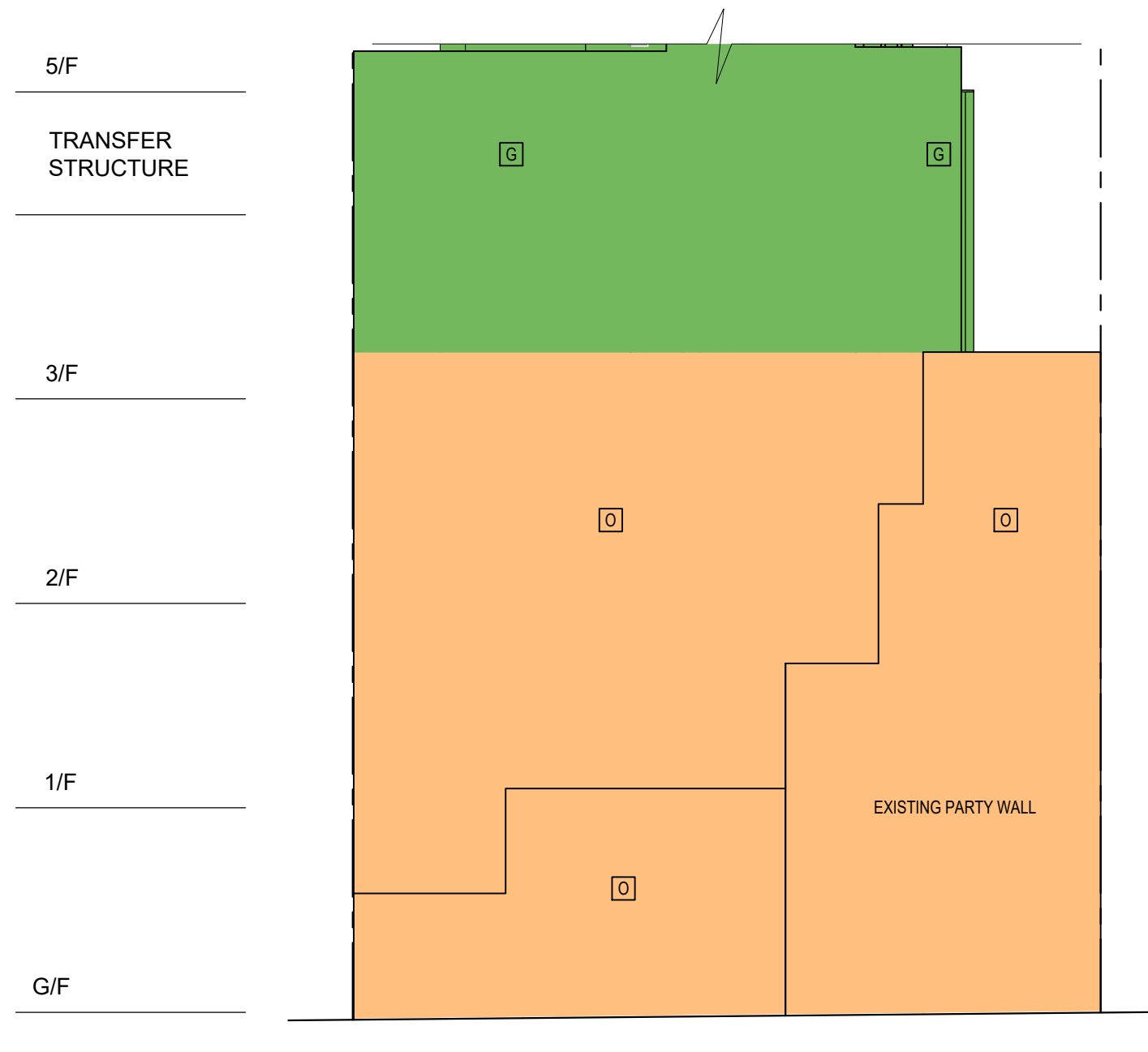
SOUTH ELEVATION
